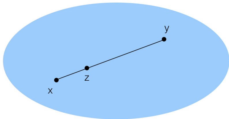
Figure 1: Convex Set
