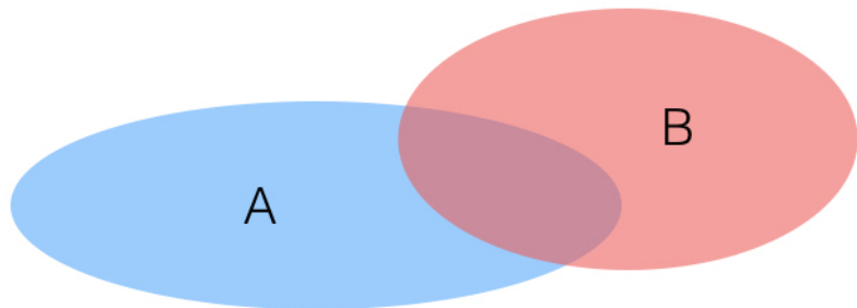
Figure 3: Intersection of A & B is convex
