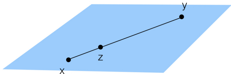
Figure 2: Convex Set
