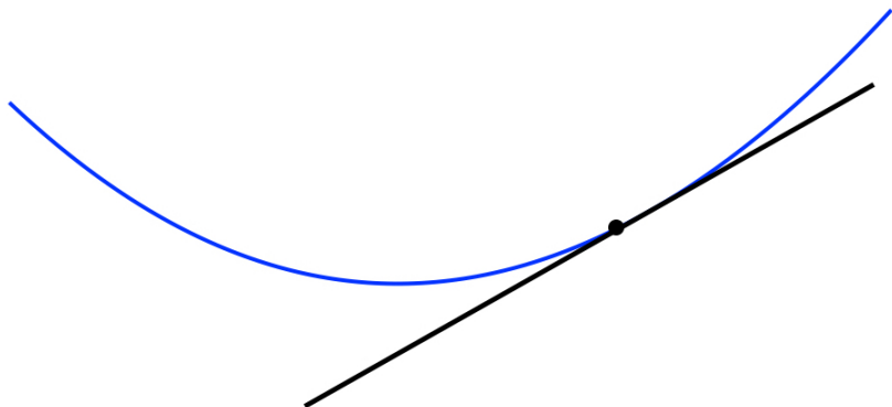
Figure 5: Best linear approximation
