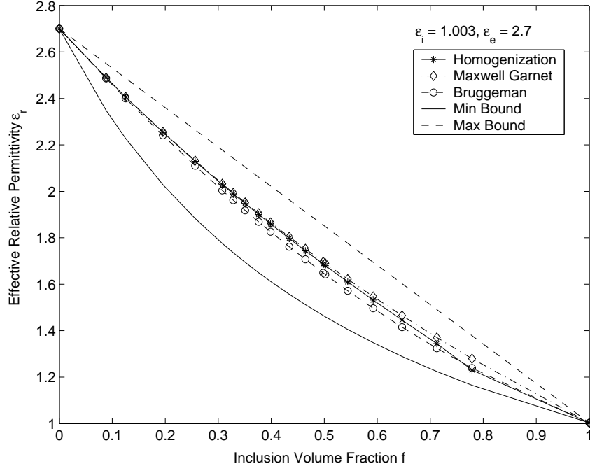
Figure 4: Effective relative permittivity distribution for random mixtures with circular microstructures.
