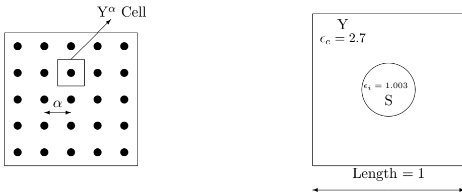
Figure 3: (left) Periodic composite material presenting a circular microstructure with periodicity \alpha . (right) The reference cell Y = [0, 1] \times [0, 1] .
