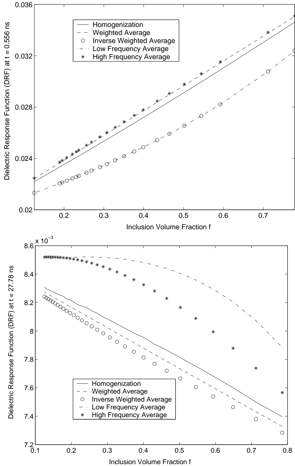
Figure 8: (top) The effective dielectric response function (DRF) \nu(t) as a function of the inclusion volume fraction for t = 0.556 ns and (bottom) t = 27.78 ns.
