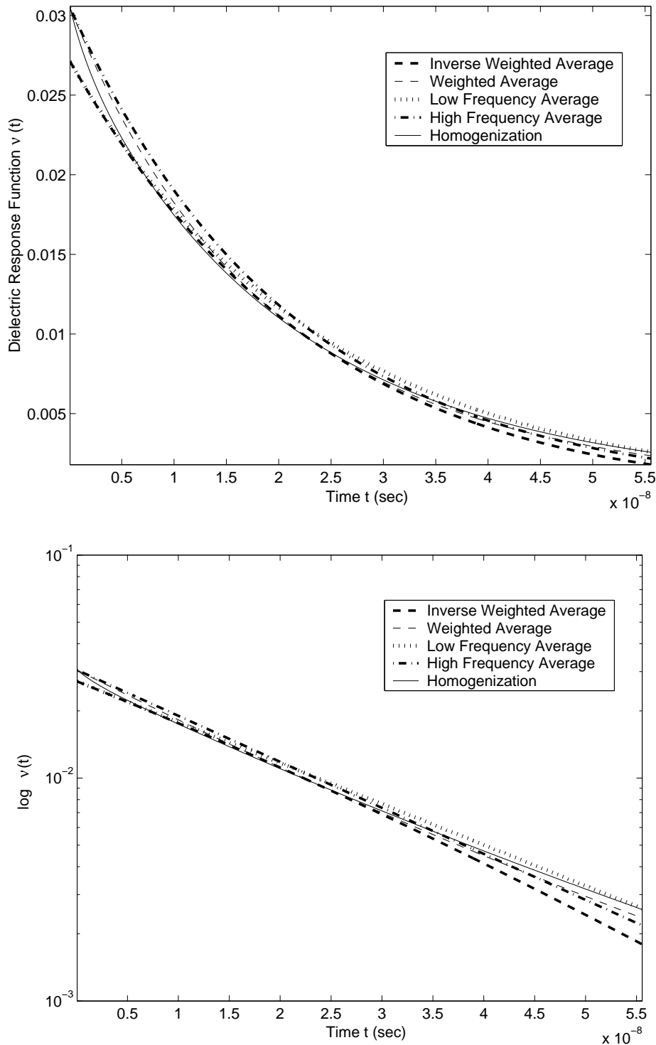
Figure 7: (top) The effective dielectric response function (DRF) \nu(t) as a function of time, for volume fraction f = 0.5 . We compare the homogenized DRF with the DRF that is a weighted average of the corresponding DRF's, as well averages that are observed in other experiments. (bottom) Semilog plot of the DRF's.
